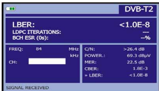
Figure 37.- Screen LBER measurement COFDM modulated signals (DVB-T2).
