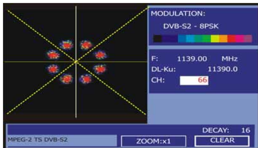
Figure 50.- Constellation Diagram. DVB-S2 (8PSK) signal.
