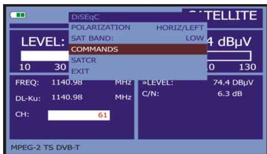
Figure 74.- DiSEqC command screen.
