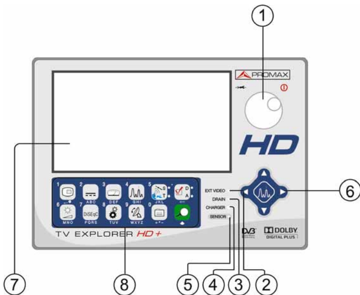
Figure 3.- Front panel.
